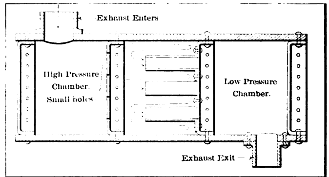
Fig. 64—Simplex type of muffer, showing three chambers, so contrived that the pressure is reduced almost to zero before the exhaust makes its exit to the atmosphere
